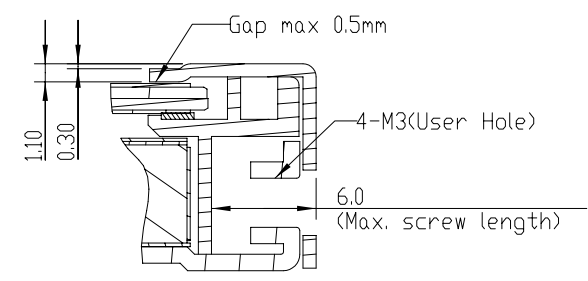
SECTION H1-H1 SCALE 3:1
